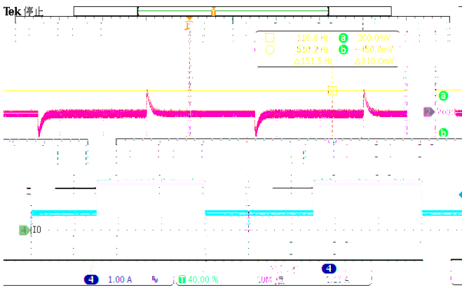
Figure 35. LoadTrans (Iload=0.5A-1.5A)
