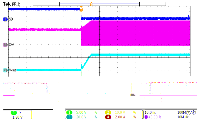
Figure 34. Shutdown remove
