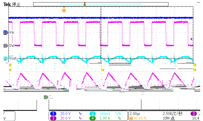
Figure 36. steady-state (Iload=2A)
