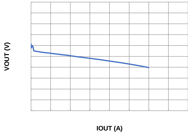
Figure 3. Load Regulation
