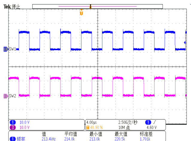
Figure 14. Full bridge
