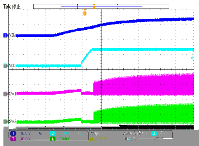
Figure 11. Power Up
