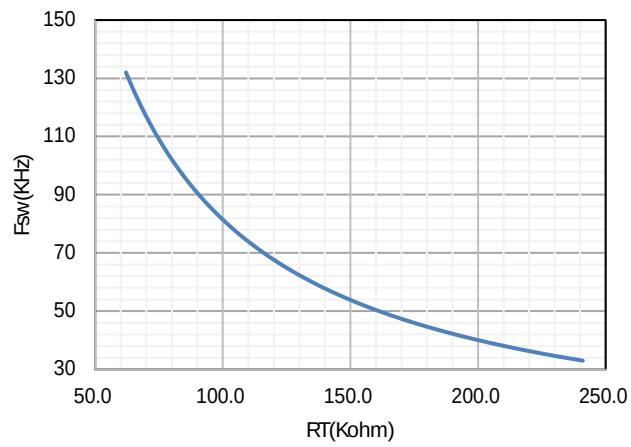
Figure 2. Clock Frequency VS FREQ Resistor
